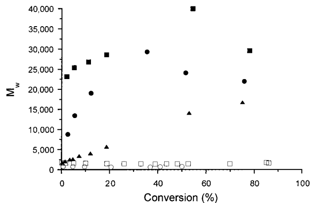
Figure 7. Evolution of the cumulative weight-average molecular weight, M_w , for styrene and methyl methacrylate polymerizations in the presence of varying amounts of CPhBF. In all cases: T = 60 °C, toluene:monomer = 2:1 (v/v), [AIBN] = 2 \times 10^{-2} mol dm -3 ; (▲) styrene, [Co(II)] 0 = 2.57 \times 10^{-4} mol dm -3 ; (●) styrene, [Co(II)] 0 = 6.22 \times 10^{-5} mol dm -3 ; (■) styrene, [Co(II)] 0 = 1.58 \times 10^{-5} mol dm -3 ; (○) methyl methacrylate, [Co(II)] 0 = 3.08 \times 10^{-5} mol dm -3 ; (□) methyl methacrylate, [Co(II)] 0 = 1.85 \times 10^{-5} mol dm -3 .
